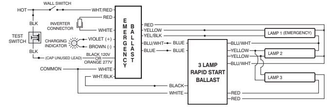
FIG 105 THREE (3) LAMP RAPID START BALLAST
