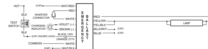
FIG 109 ONE (1) 17-215 W LAMP WITHOUT AC BALLAST
