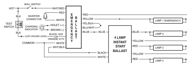
FIG 121 FOUR (4) LAMP INSTANT START BALLAST
