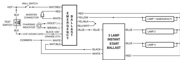
FIG 106 THREE (3) LAMP INSTANT START BALLAST
