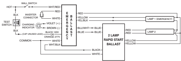
FIG 124 TWO (2) LAMP RAPID START BALLAST
