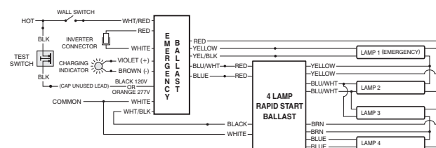
FIG 120 FOUR (4) LAMP RAPID START BALLAST
