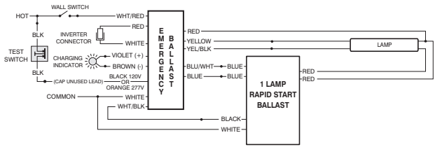
FIG 099 ONE (1) LAMP RAPID START BALLAST
